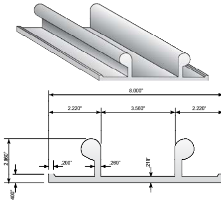
Cross Section of Heavy-Duty Vertical Rail
