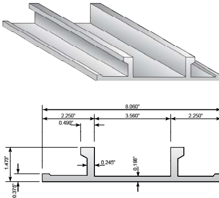
Cross Section of Standard Vertical Rail
